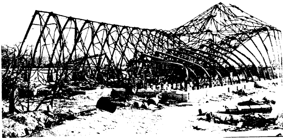
Figure 5.29. Single-story, light steel-frame building (0.80 mile from ground zero at Hiroshima); partially damaged by blast and further collapsed by subsequent fire.
