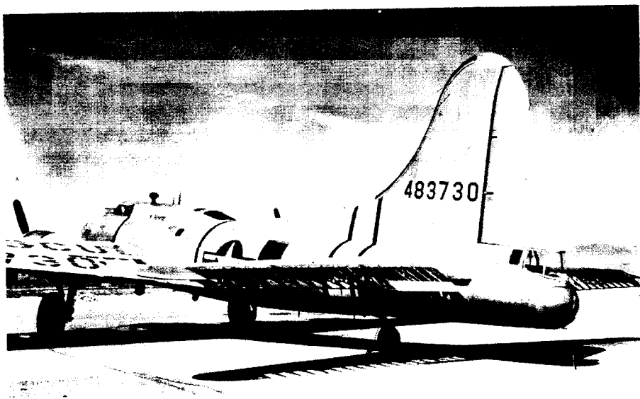
Figure 5.95b. Aircraft after tail exposed to a nuclear explosion (2.4 psi peak overpressure).
