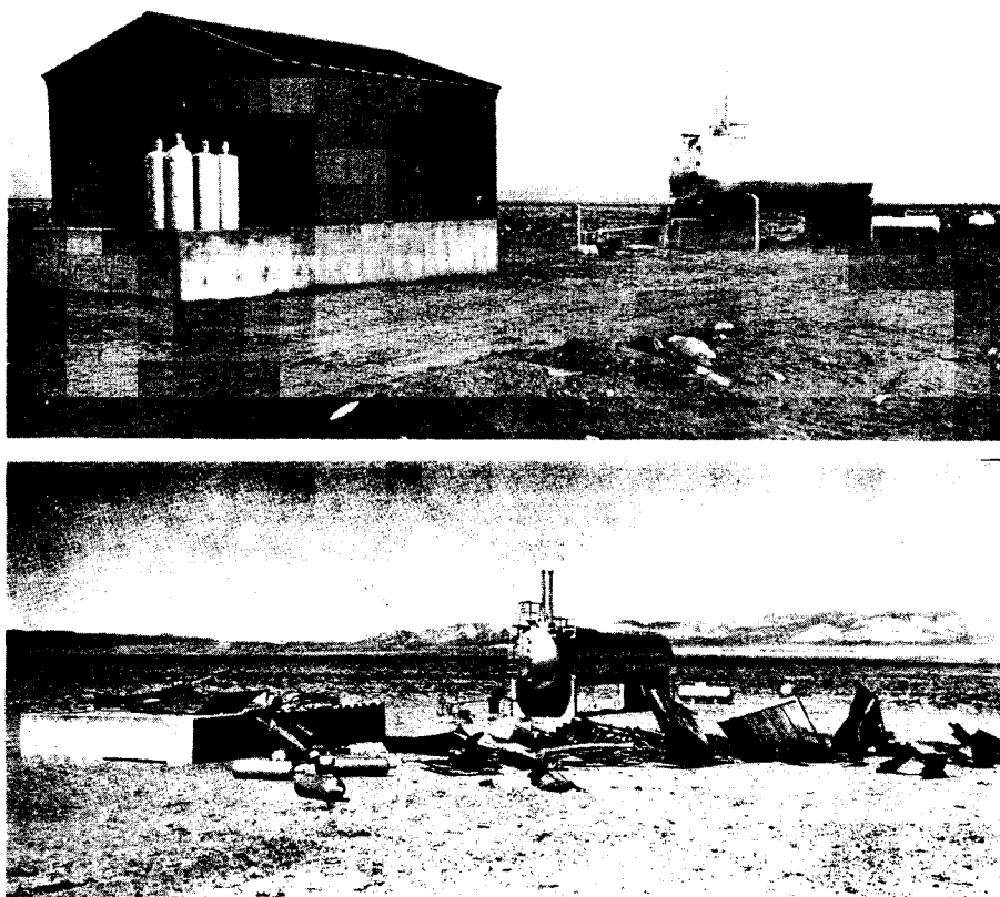
Figure 5.120. Upper photo: LP-gas bulk storage and filling plant before a nuclear explosion. Lower photo: The plant after the explosion (5 psi peak overpressure).
